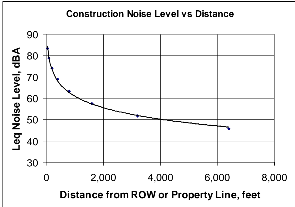
FIGURE A08-1 Estimated Construction Noise Levels
