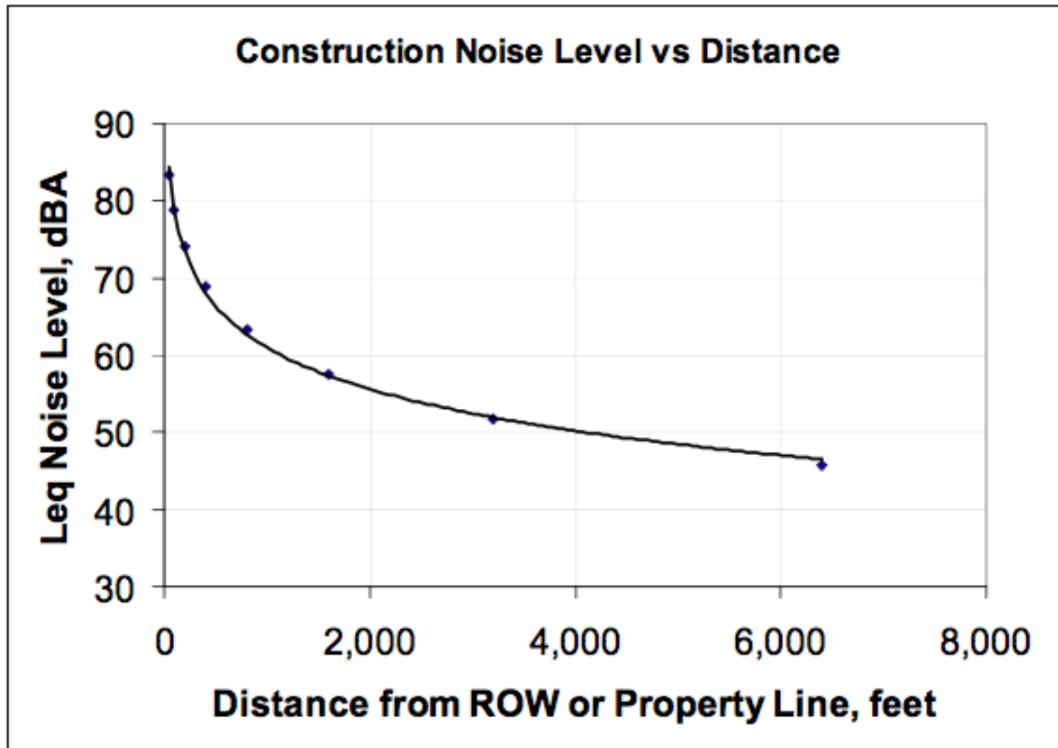
FIGURE 8-1 Estimated Construction Noise Levels
