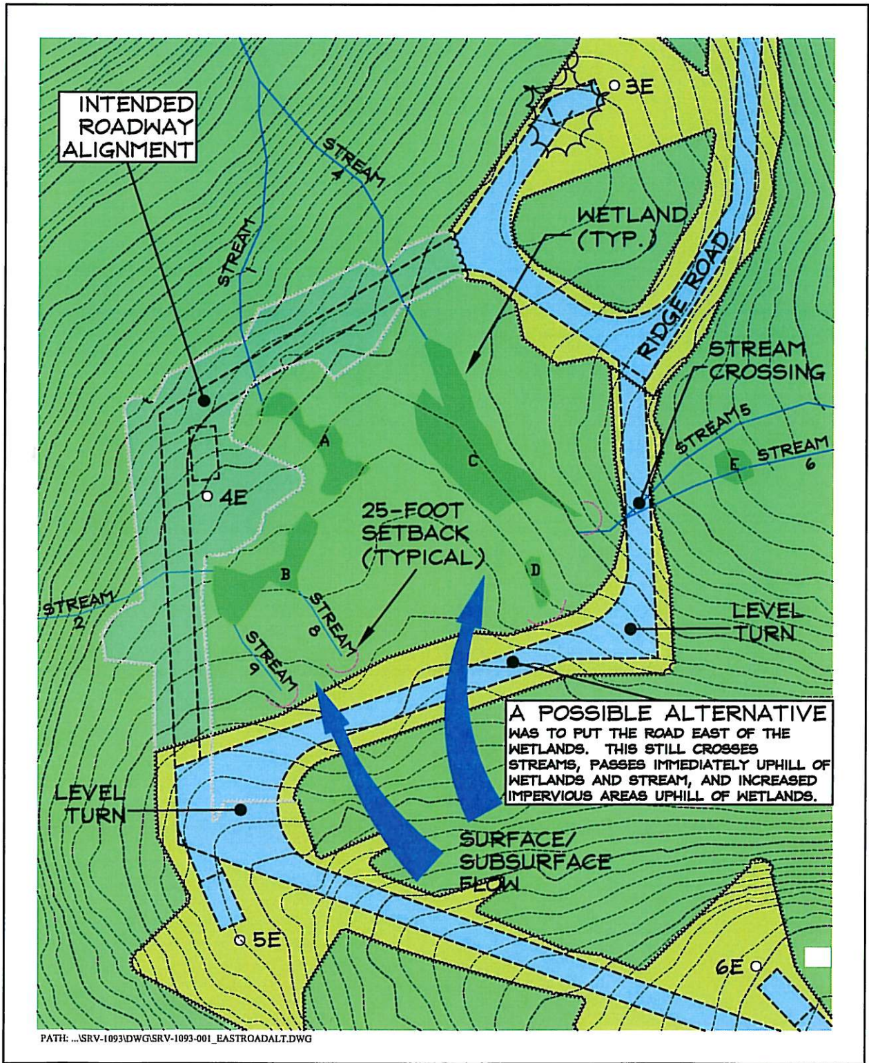
Exhibit DFLD-JK-5 Road Layout Alternative - East Ridge Wetlands Scale: 1" = 200 feet
