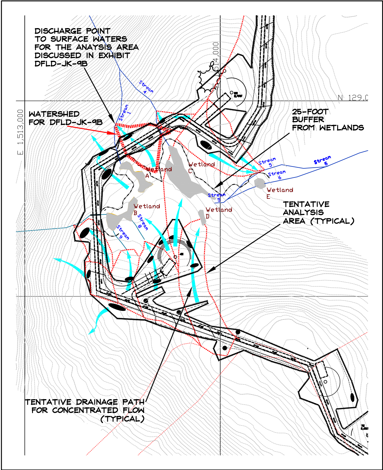
Exhibit DFLD-JK-Rev9B Figure One - Turbine 4E Drainage Area Not To Scale
