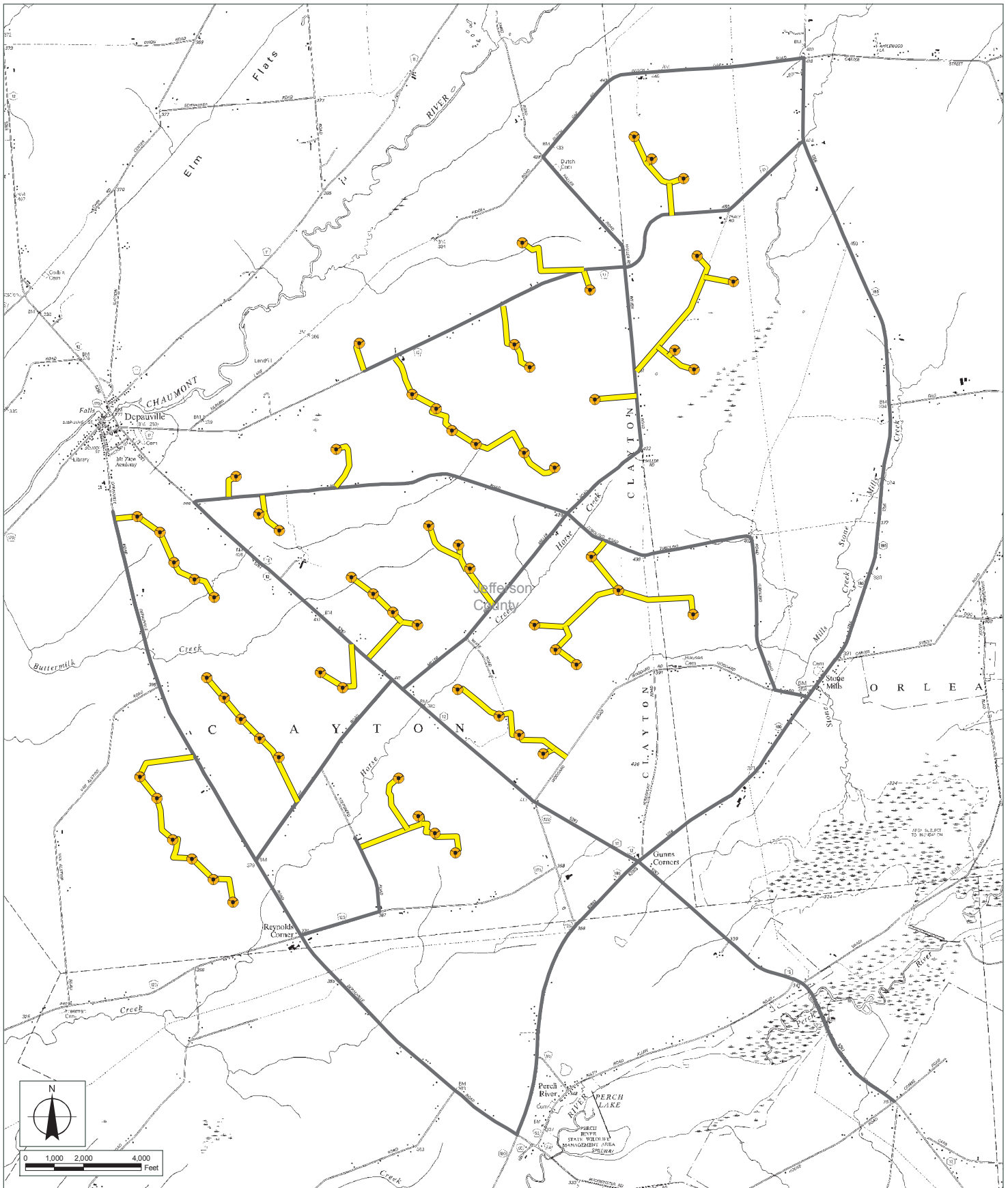
Horse Creek Wind Farm Towns of Clayton and Orleans - Jefferson County, New York Figure 12: Preliminary Transportation Routing
